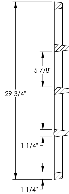
SECTION B-B
